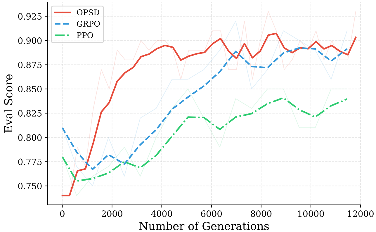
Qwen3-4B / Characterbench — Eval Score
