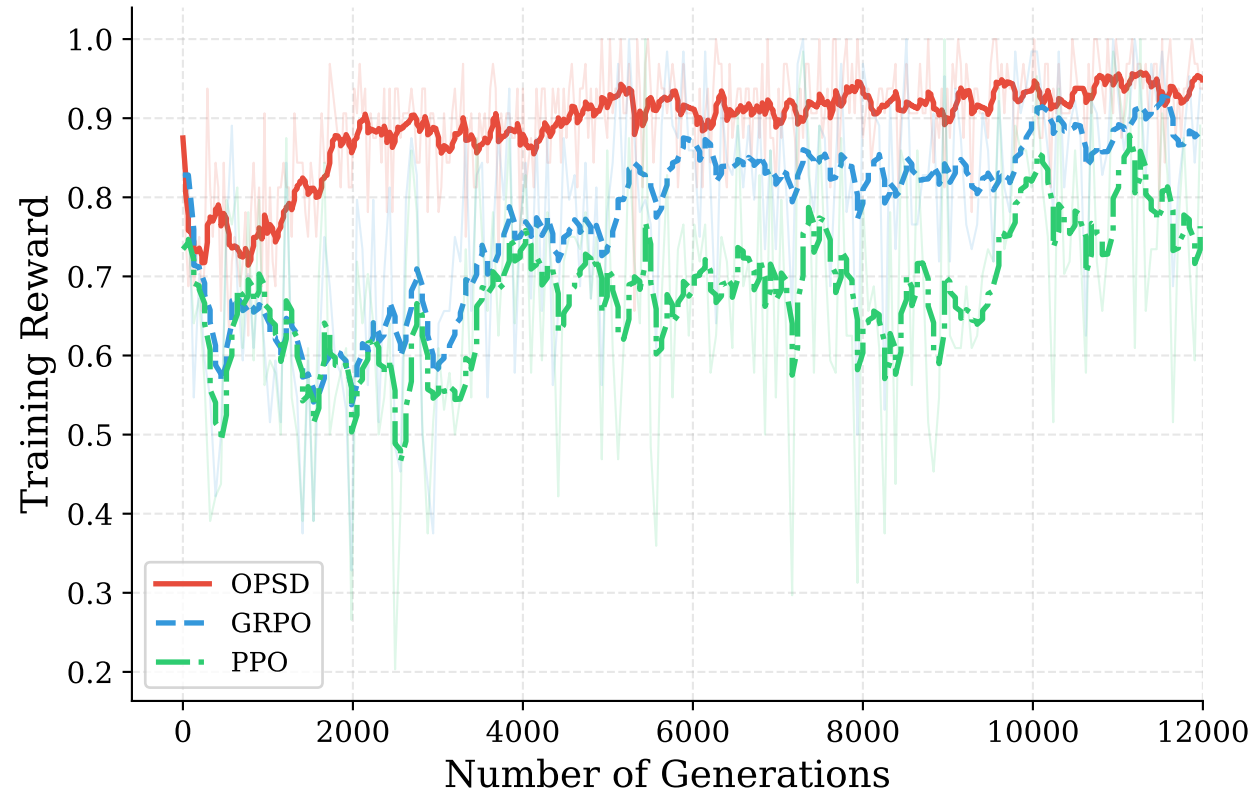
Qwen3-4B / Characterbench — Training Reward
